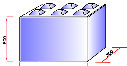
TYPE A3 (gew: 1800 kG)
